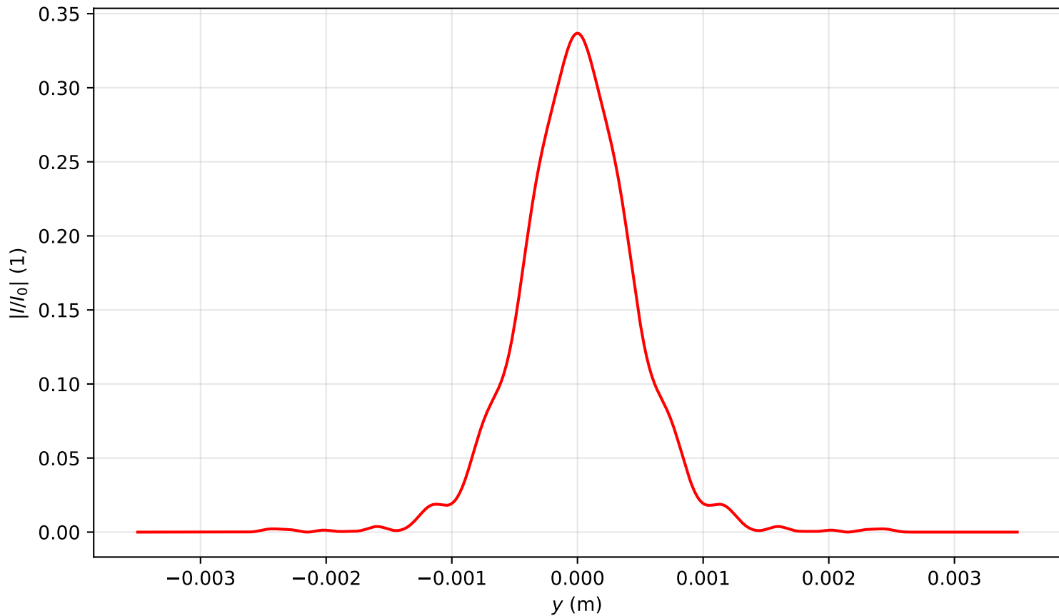
Intensity profile I(x = 0, y, z = 2.866)/I_0 , P_{in}=1.0P_{cr} , artificial time
